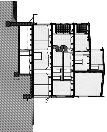
A.MMG_498 Conversion CP6, Papierl-Areal_3_Detailsection Detailsection 1110
