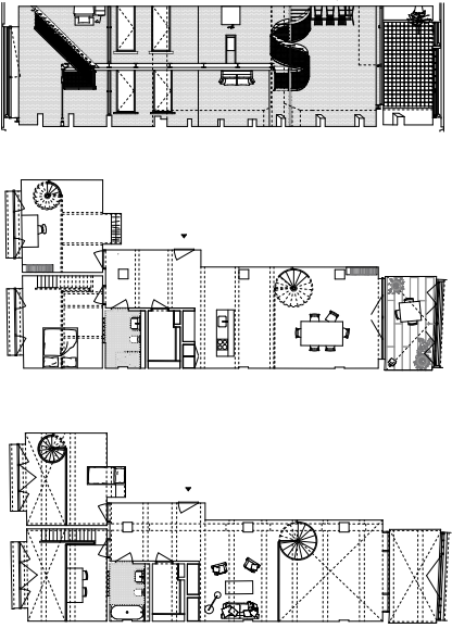
A.MMG_498 Conversion CP6, Papierl-Areal_3_Detail Flat Detail Plan 1110
